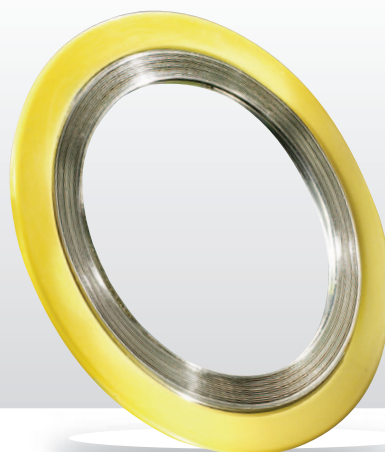
Thermiculite® 835 Spiral Wound Gasket with Heat Treated Inconel X-750 Winding
